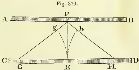
Action of Intercostal Muscles.
